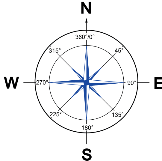
Figure 22: Wind rose
