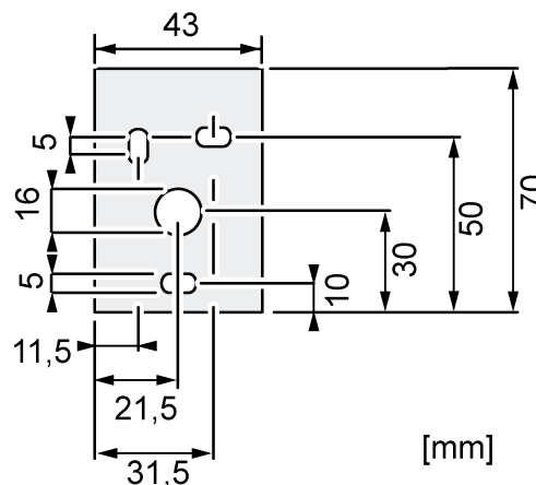
Figure 5: Template of drillholes and cable penetration
